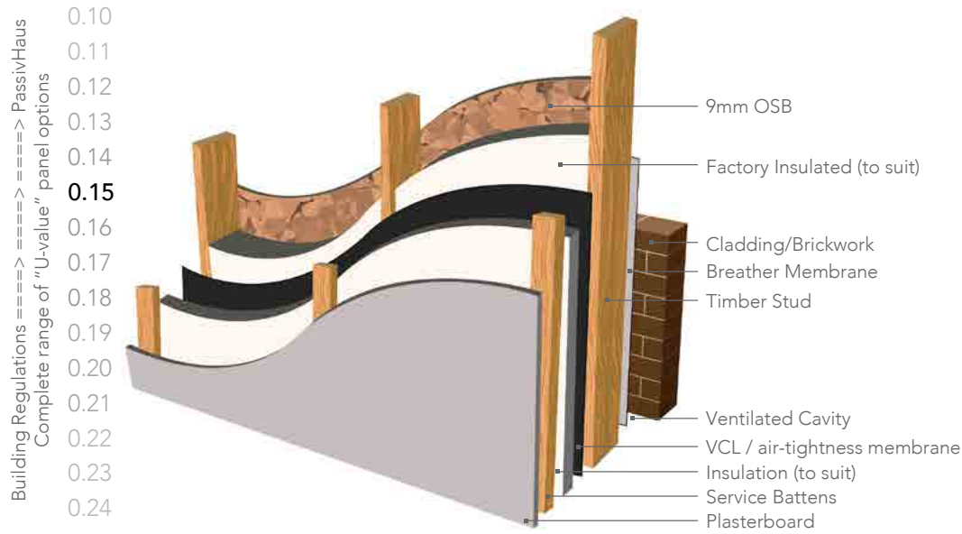
Typical timber frame wall section
