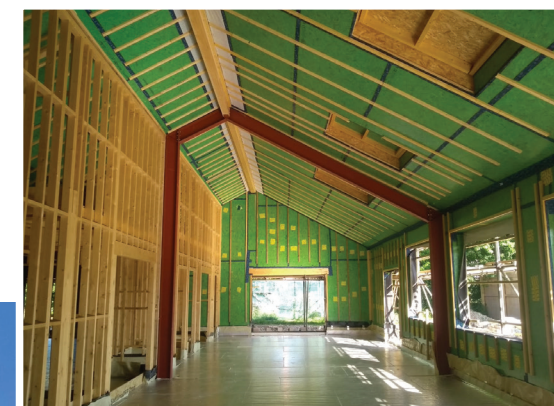
The Passivhaus 'Museum of Speed' in Pendine, Wales
